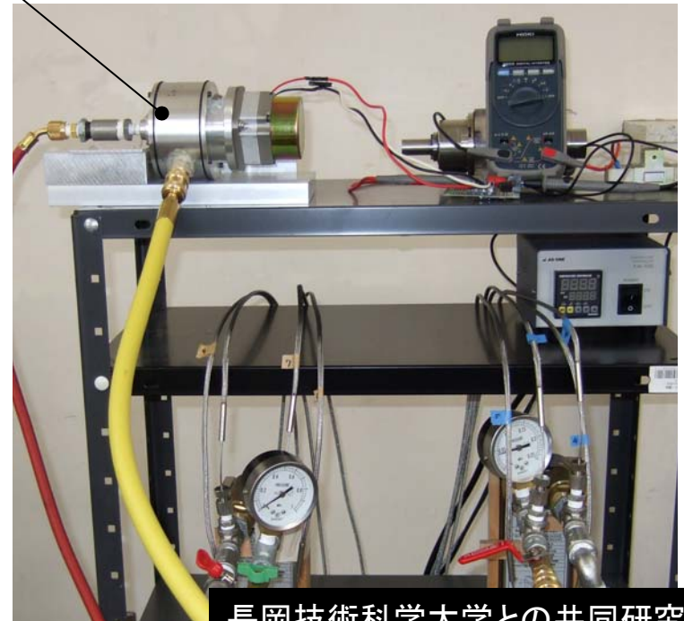
Scroll Turbine / Expander
